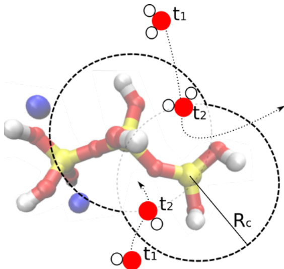
Figure 1. A schematic representation of the algorithm developed to analyze the local environment around silicates during the dissociation by sodium hydroxide. The silicon atoms are represented in yellow, oxygen atoms in red, hydrogen atoms in white, and sodium atoms in blue.
