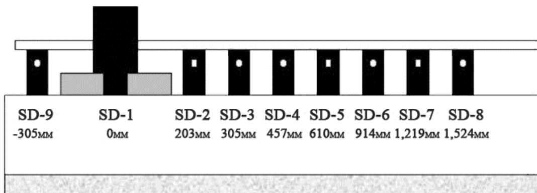
Figure 4-2: Fixed sensor configuration for LTPP FWD testing [32].
