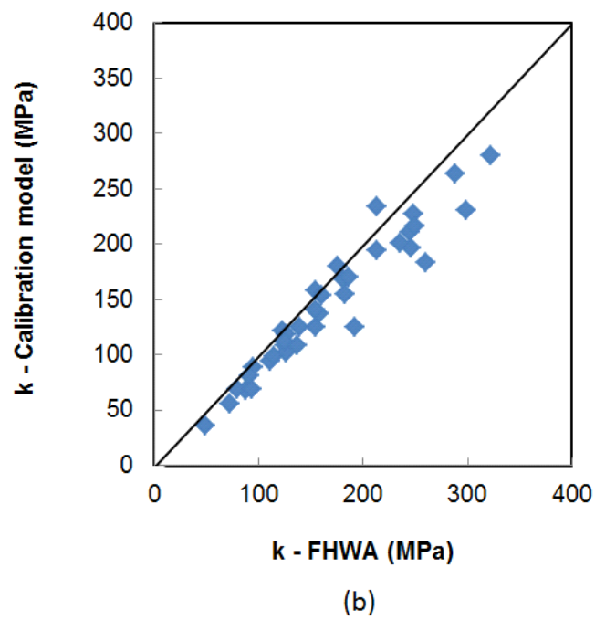
Figure 4-8: Comparison of top layer modulus E and subgrade modulus k values obtained from calibration model and from the LTPP reported data [28].
