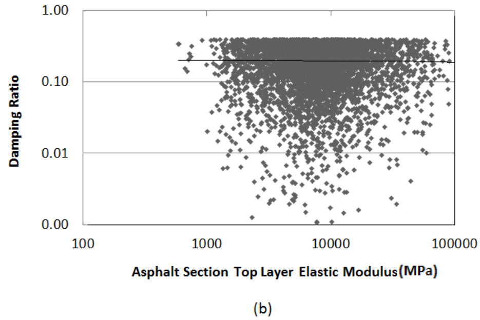
Figure 4-14: Cross-plot of the damping ratio \zeta vs. top layer elastic modulus E of (a) concrete (b) asphalt sections showing no correlation between the two elements.
